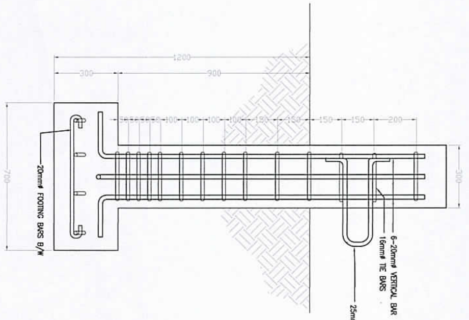
CONCRETE ANCHOR POST SECTION DETAILS SCALE 1:20 MS
